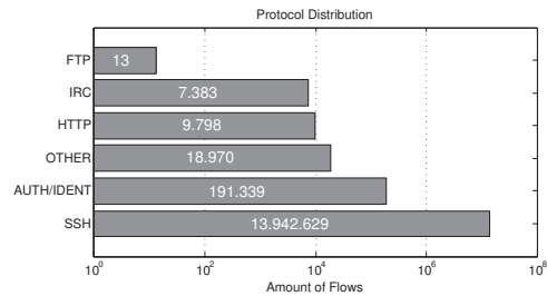
Fig. 2. The protocol distribution of the original training set.
