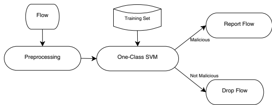
Fig. 1. The high-level view on the proposed approach for an inductive NIDS.
