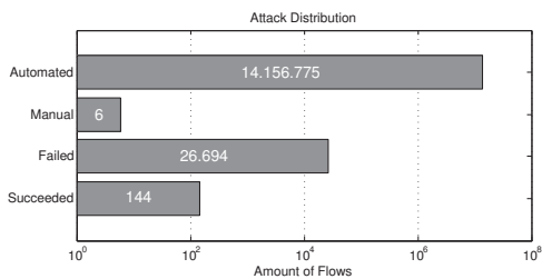
Fig. 3. The attack types of the original training set.
