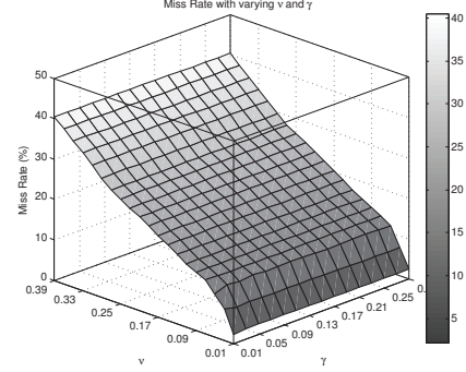
Fig. 5. Relationship between the varying parameters \nu and \gamma and the miss rate during the fine grained grid search.
